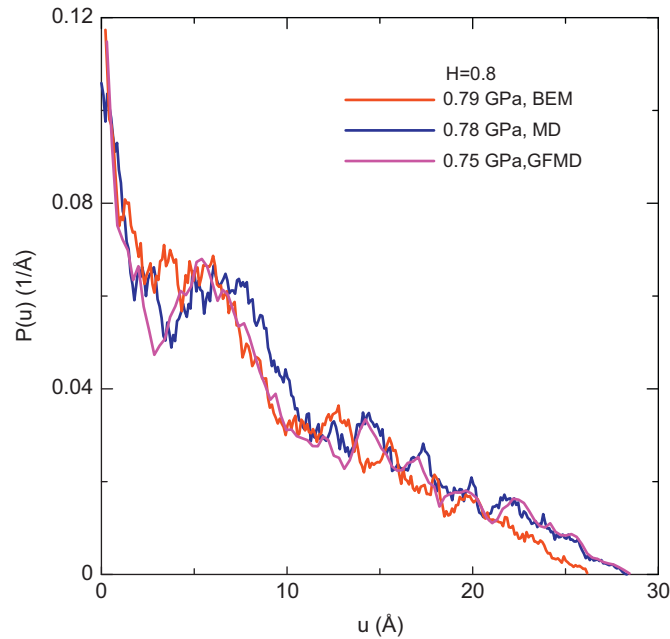
Fig. 9. Probability distribution P(u) of interfacial separations u , obtained using the BEM, MD and GFMD methods for p=0.79 , 0.78 and 0.75 GPa, respectively.
