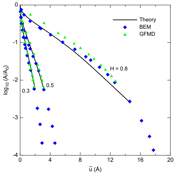
Fig. 12. The contact area A/A_0 as a function of average interfacial separation \bar{u} for the H=0.3, 0.5 and 0.8 surfaces.
