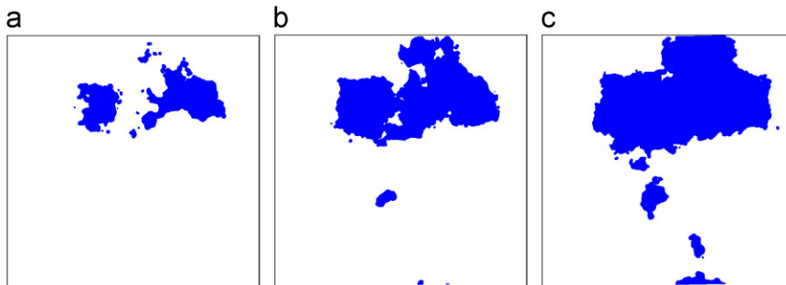
Fig. 8. Contact morphologies predicted by a bearing area model for the same “true” contact area A values as in Fig. 7 but where long-range elastic coupling has been neglected. (a) A/A_0=0.066 . (b) A/A_0=0.161 . (c) A/A_0=0.238 .
