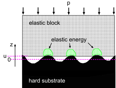
Fig. 1. An elastic block squeezed against a rigid rough substrate. The separation between the average plane of the substrate and the average plane of the lower surface of the block is denoted by u . Elastic energy is stored in the block in the vicinity of the asperity contact regions.
