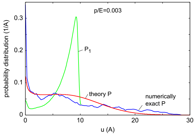
Fig. 11. Probability distribution P(u) for the squeezing pressure p=0.003E obtained in a numerically exact calculation (blue curve), and by applying the theoretical result from (Eq. (16)) (red curve). Also shown is the theory prediction (Eq. (17)) for the distribution P_1(u) of boundary-line averaged interfacial separations (green curve). (For interpretation of the references to color in this figure legend, the reader is referred to the web version of this article.)
