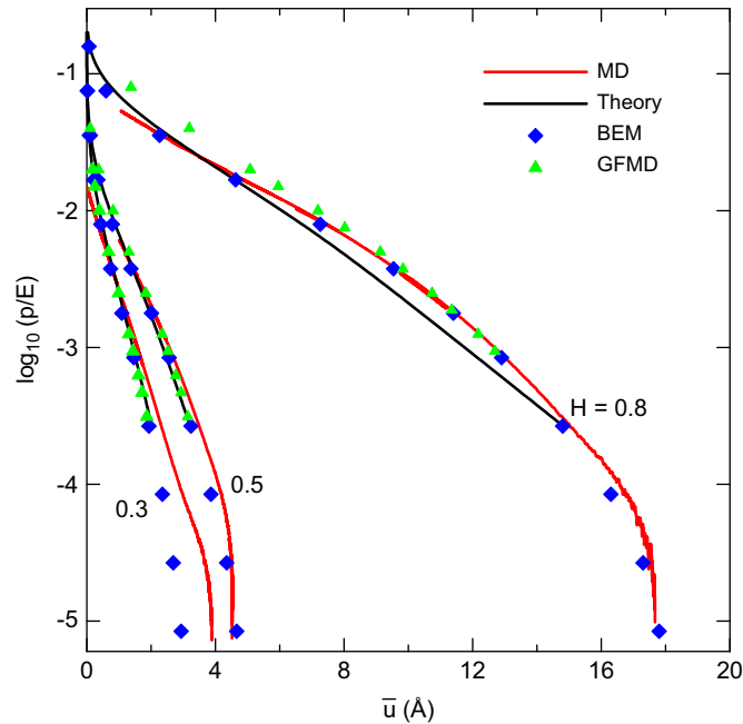
Fig. 5. The relation between the applied squeezing pressure p and the average interfacial separation \bar{u} . (For interpretation of the references to color in this figure legend, the reader is referred to the web version of this article.)
