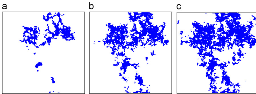
Fig. 7. Contact morphologies for the H=0.8 surface at three different contact pressures; (a) p=0.0032E , (b) p=0.0080E and (c) p=0.0120E when long-range elastic deformations are considered. The fractional contact areas are A/A_0=0.066 , 0.161 and 0.238 , respectively.
