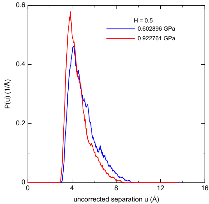
Fig. 6. Distribution of interfacial separations for the substrate with H=0.5 obtained in classical MD simulations.
