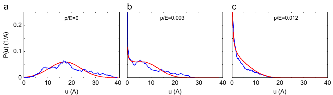
Fig. 10. Probability distribution P(u) for several squeezing pressure values. The red line corresponds to the theoretical predictions and the blue to numerical simulations (in (a) and (c) using BEM and in (b) using GFMD). (For interpretation of the references to color in this figure legend, the reader is referred to the web version of this article.)
