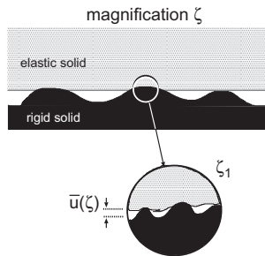
Fig. 3. An asperity contact region observed at the magnification \zeta . It appears that complete contact occurs in the asperity contact region, but when the magnification is increased to the highest (atomic scale) magnification \zeta_1 , it is observed that the solids are actually separated by the average distance \bar{u}(\zeta) .
