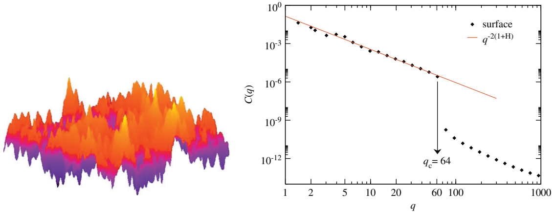
Fig. 4. Graphical representation of a rough topography with Hurst exponent H=0.3 and its corresponding height–height correlation function C(q) = \langle |h(\mathbf{q})|^2 \rangle in Fourier space. The surface topography was created using a Fourier filtering technique and a hard cutoff q_c=64 was imposed to it in Fourier space (in units of 2\pi/L , where L is the linear size of the simulation cell). The continuous line represents the ideal algebraic scaling expected for the height–height correlation function of such a surface.
